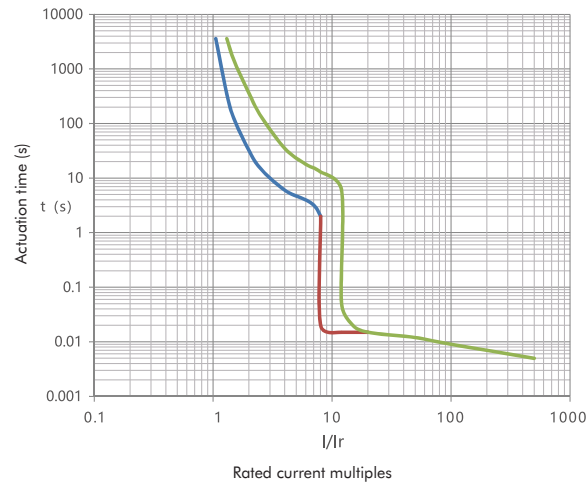
Tripping curve
